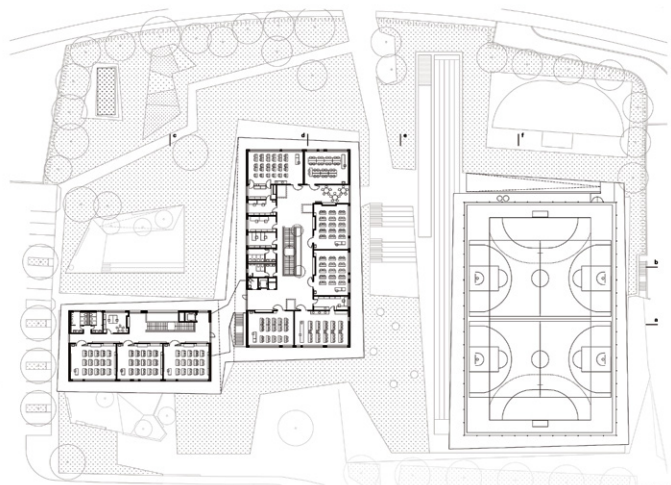
floor 2.kata | +8.00
