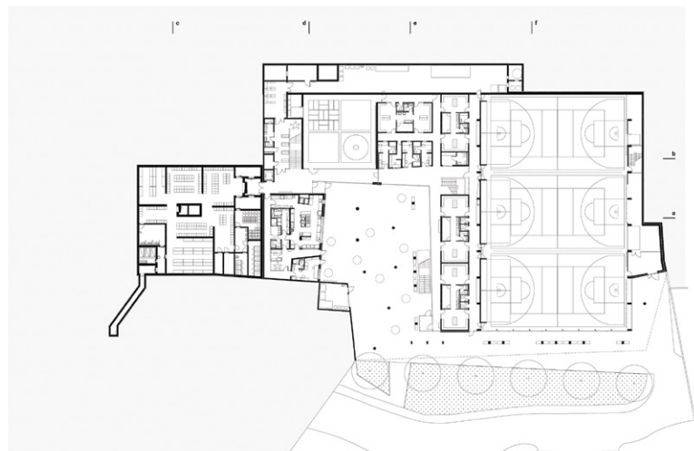
floor podruma | -3.30
